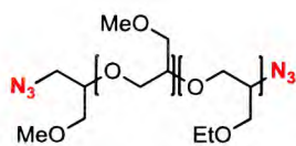
\text{N}_3\text{-LPG-N}_3
