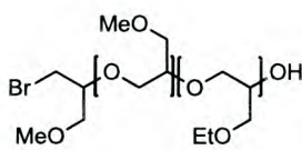
Br-LPG-OH
