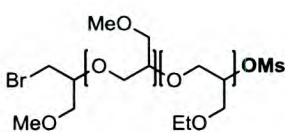
Br-LPG-OMs
