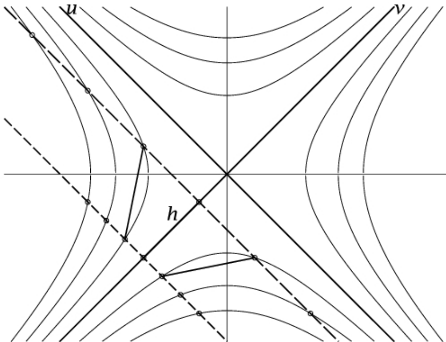
FIG. 2. Two dimensional Minkowski space: x^0 and x^1 are the vertical and horizontal axes. A few orbits of the Lorentz group are shown, including the u and v axes. Misner space \mathcal{M}_2 can be regarded as the strip between \ell (null dashed-line) and \mathcal{B}\ell (null line in long dashes) with points in \ell identified with their image under \mathcal{B} in \mathcal{B}\ell (this is the t -axis in Fig.1). Some of these pairs of identified points are marked with circles. The three geodesic segments shown are, from left to right, time-like, null and space-like; they become closed geodesics in \mathcal{M}_2 . The closed null geodesic h at t = 0 ( u = 0 ) separates the non causal region M_2^> above it ( t > 0, u > 0 ) from the causal region M_2^< below ( t < 0, u < 0 ).
