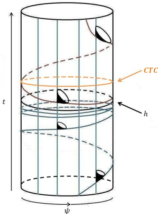
FIG. 1. Two dimensional Misner space:
