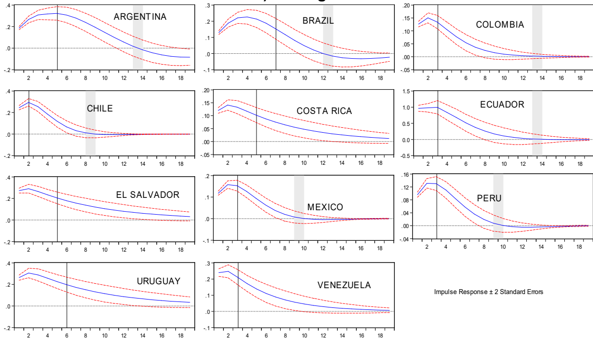
Figure 4: Impulse Response of the SRER1 (Non-tradable to Tradable Price Indexes Ratio) Misalignments
