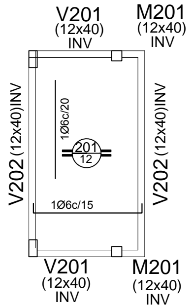
BASE TANQUE
