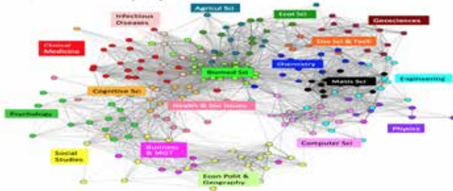
Figure 2. Global science map based on citing similarities among ISI Subject Categories (2007).
