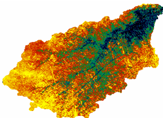
Figura 6 DEM (ASTER)
